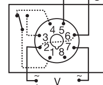
8-Pin SPDT
