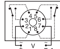
8-Pin DPDT
