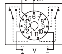
11-Pin DPDT
