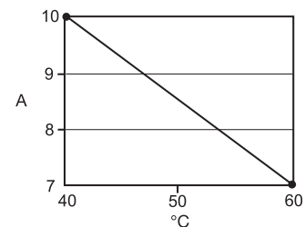
Output Current / Ambient Temp.
